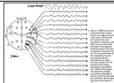
Figure 1.26 - EEG Display
